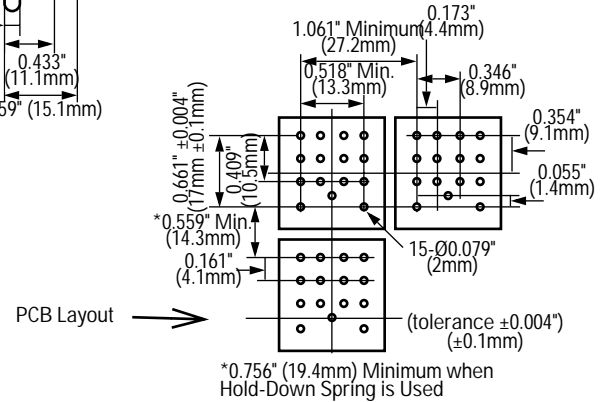
Terminal Arrangement
